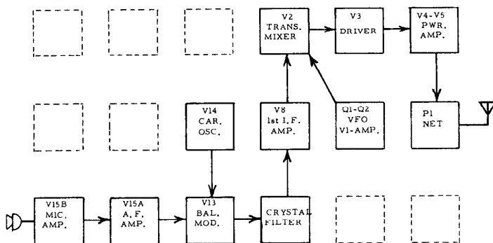
FIGURE 2 BLOCK DIAGRAM, TRANSMIT MODE
